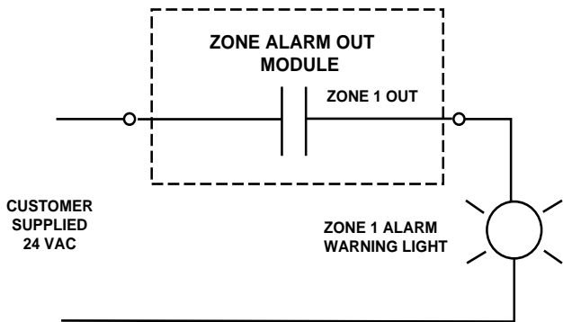
Typical Customer Connections Figure 2
